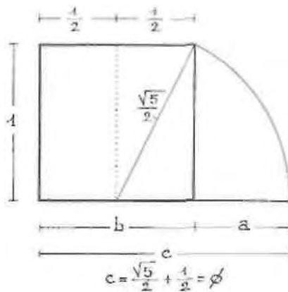
Fig. 7. Geometrical construction of \Phi (multiplacative form);.
